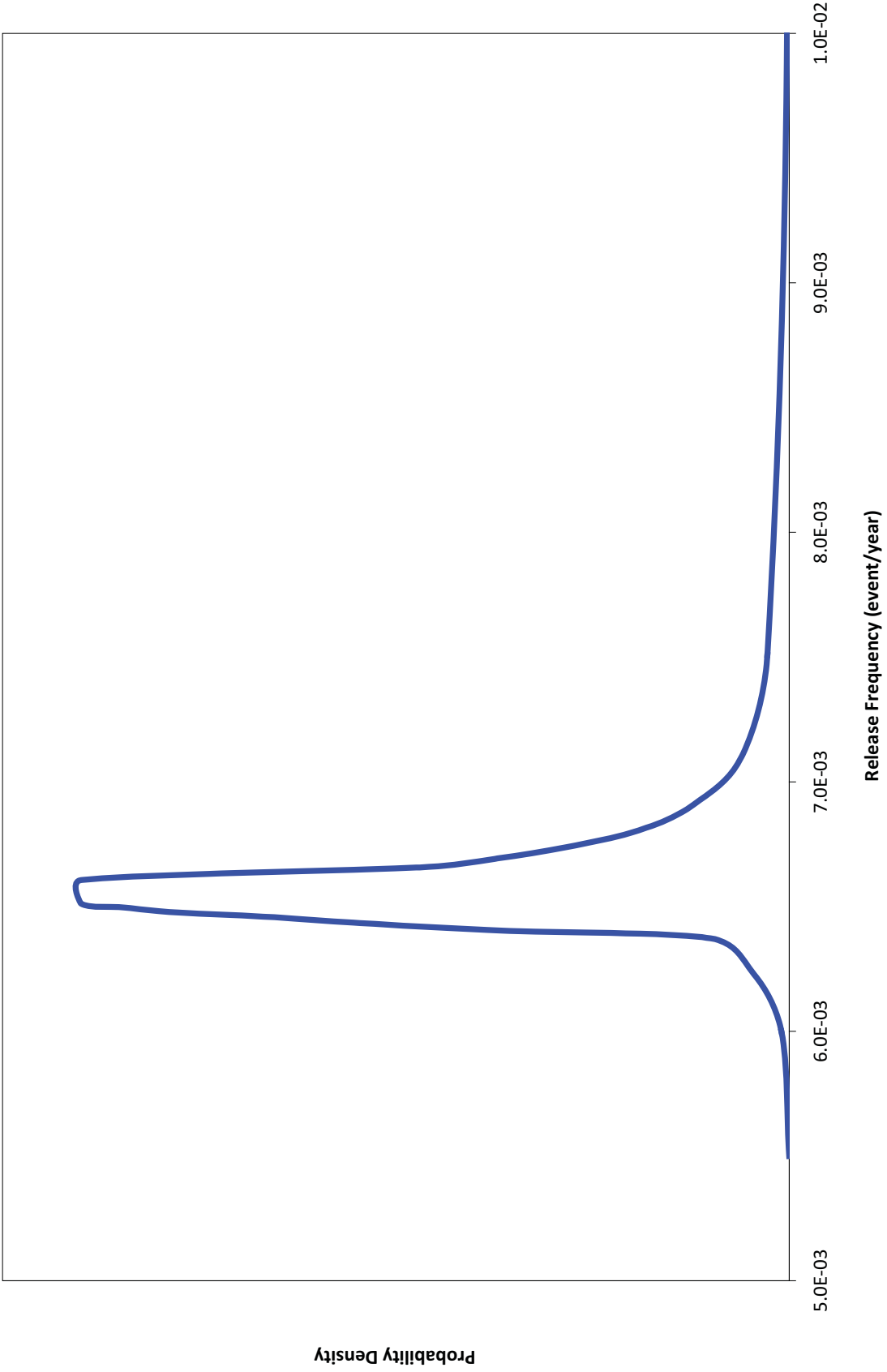
Figure 13.1-2. Release Frequency for Exceeding a Dose of 0.1 mrem in 1 Year, Probability Density Format
